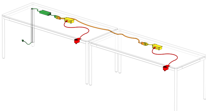
C. Daisy-chained Power between 2 Tables
