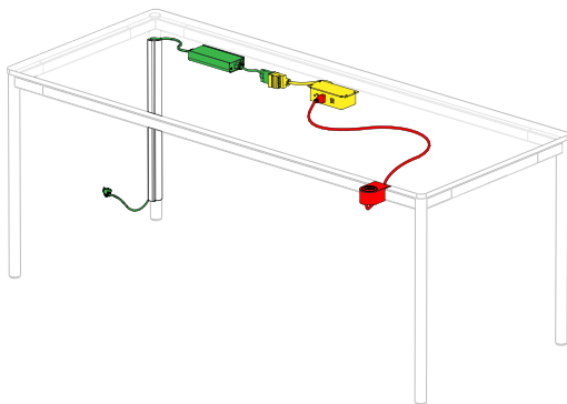
B. Power Module plugged into an Undersurface Power "Duo"
