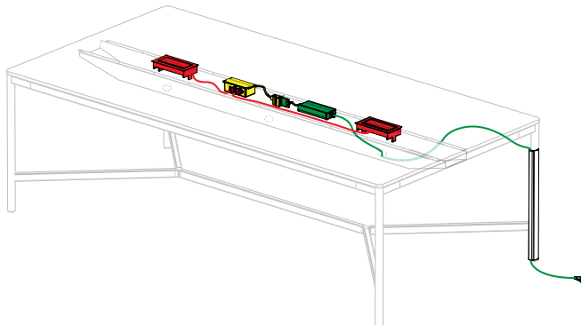
G. Community Table XRay Power Overview
